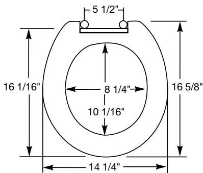
TOP-TITE® HINGES FEATURE NO-SLIP WASHER
